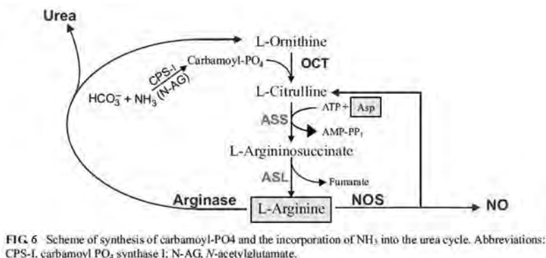
Figure 7: Metabolic Pathway for NO production.
